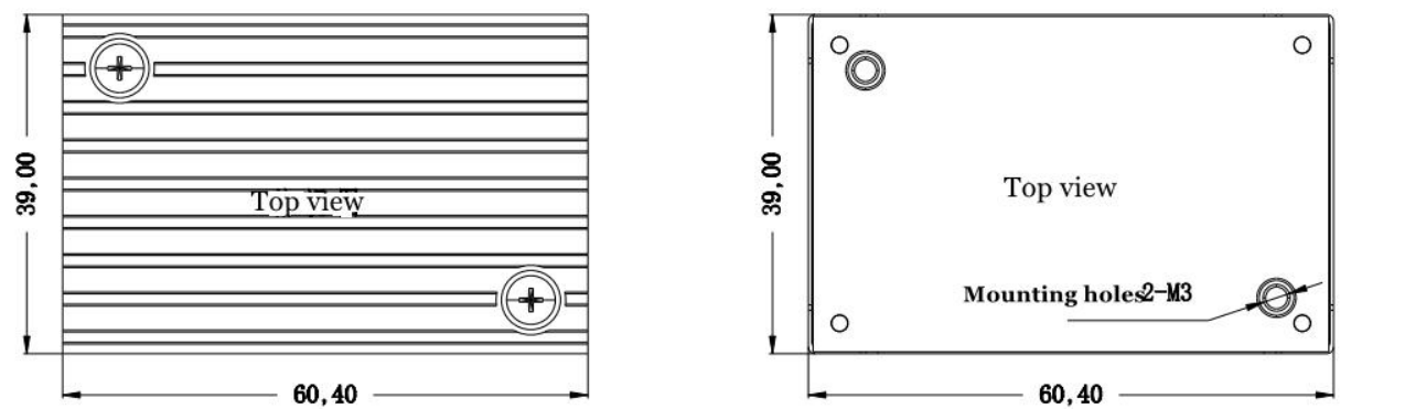
Standard+Heatsink
